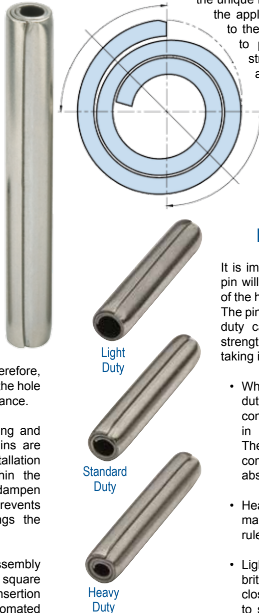
SPIROL ® Coiled Spring Pins are available in three “duties” to enable the designer to choose the optimum combination of strength, flexibility and diameter to suit different host materials and application requirements.
